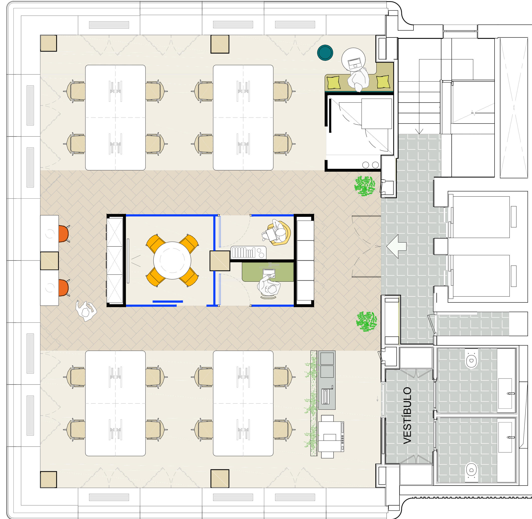
Standard floorplate example layout 221.36 sqm
