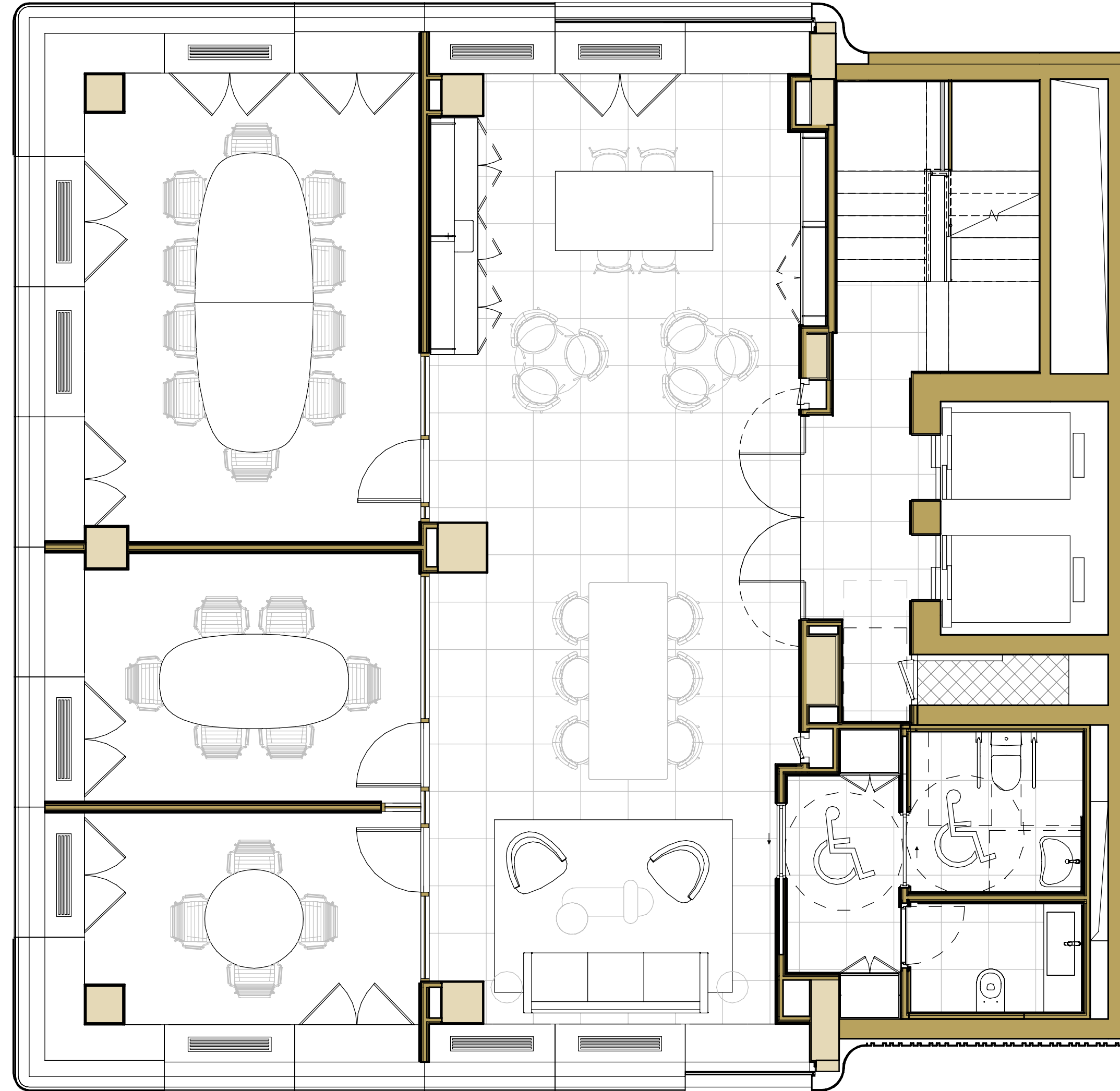
Floor 1 221.36 sqm
